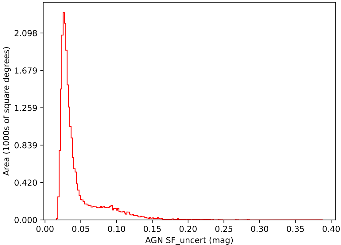
too_elab_r128_d2_griz_v3.4_10yrs i band: AGN SF_uncert
