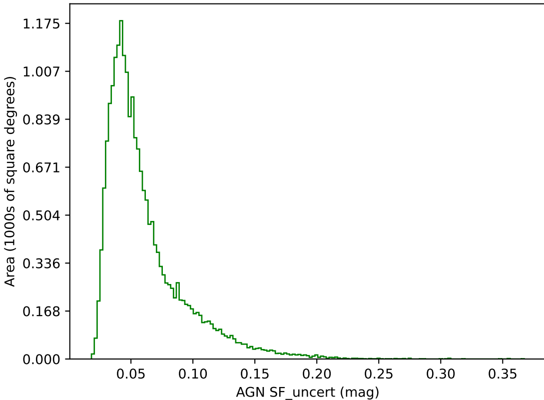
too_elab_r128_d2_griz_v3.4_10yrs g band: AGN SF_uncert
