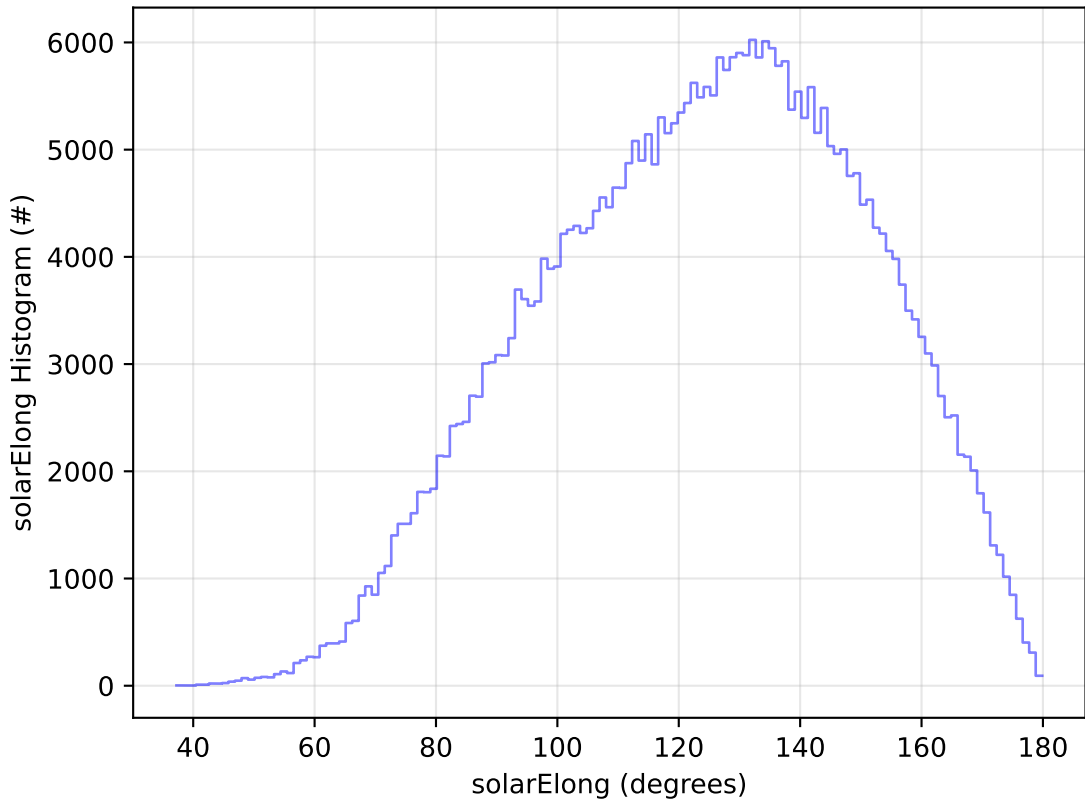
too_elab_r128_d2_griz_v3.4_10yrs WFD y band: solarElong Histogram
