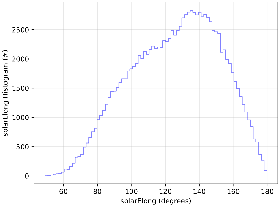
too_elab_r128_d2_griz_v3.4_10yrs WFD u band: solarElong Histogram
