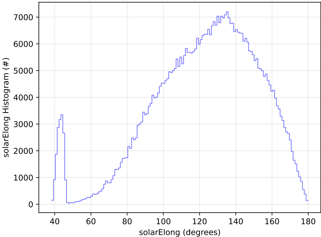
too_elab_r128_d2_griz_v3.4_10yrs WFD r band: solarElong Histogram
