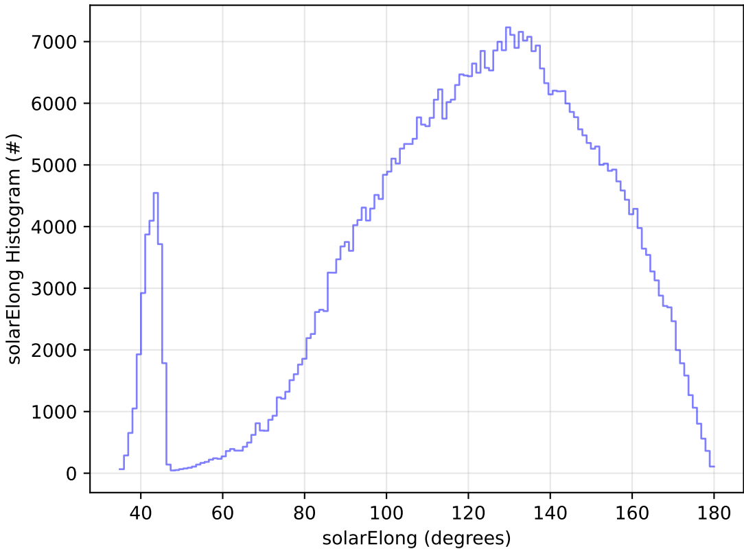
too_elab_r128_d2_griz_v3.4_10yrs WFD i band: solarElong Histogram
