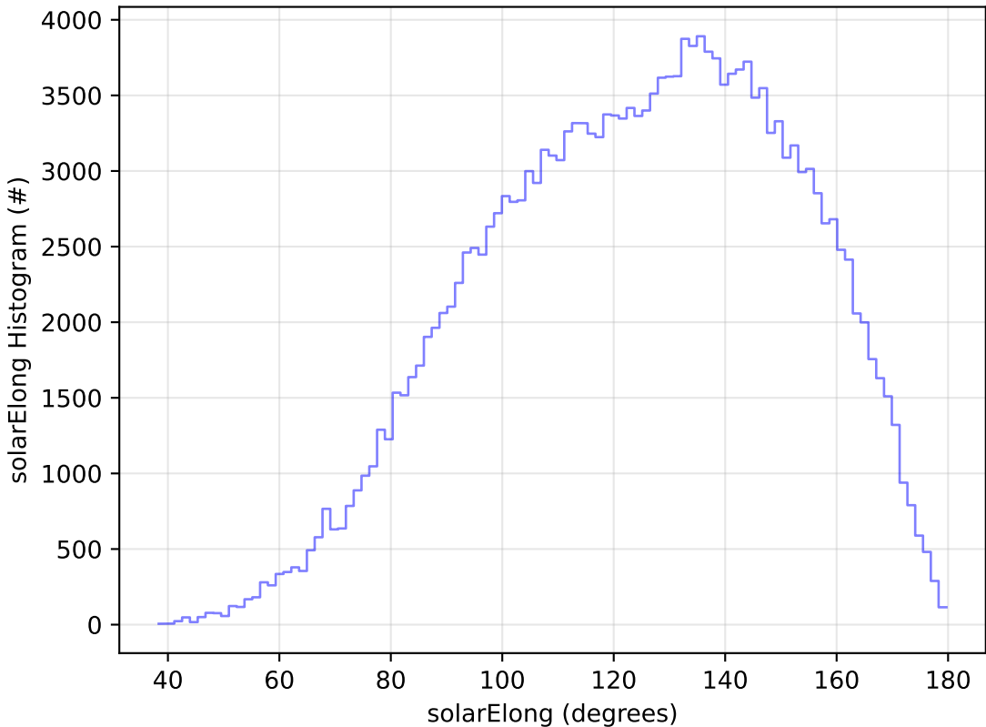
too_elab_r128_d2_griz_v3.4_10yrs WFD g band: solarElong Histogram
