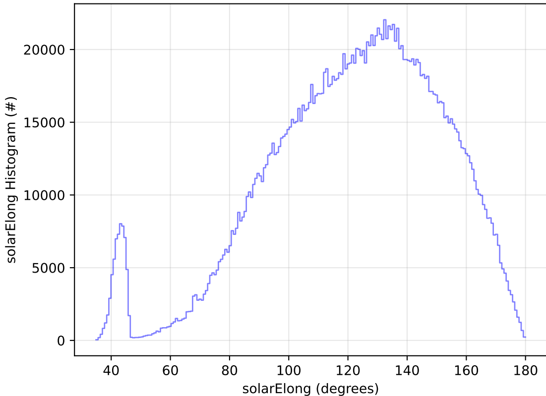
too_elab_r128_d2_griz_v3.4_10yrs WFD all bands: solarElong Histogram
