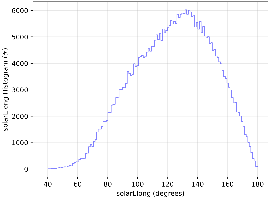
too_elab_r128_d2_griz_v3.4_10yrs All sky y band: solarElong Histogram
