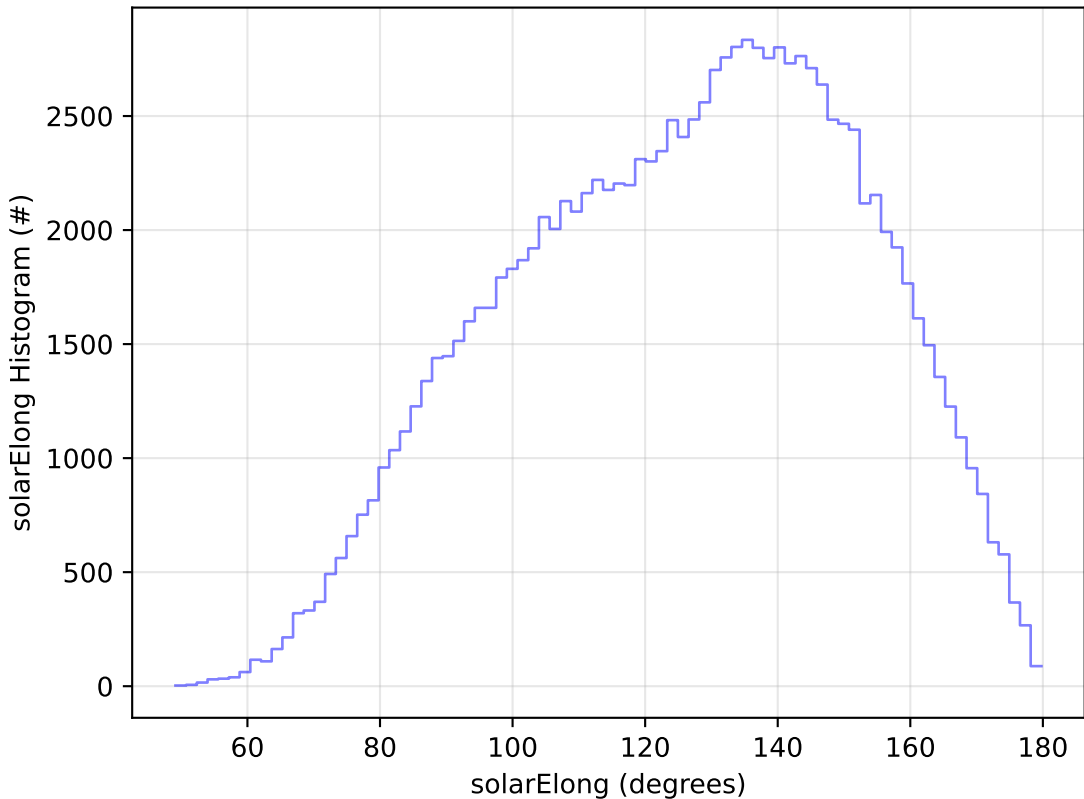
too_elab_r128_d2_griz_v3.4_10yrs All sky u band: solarElong Histogram
