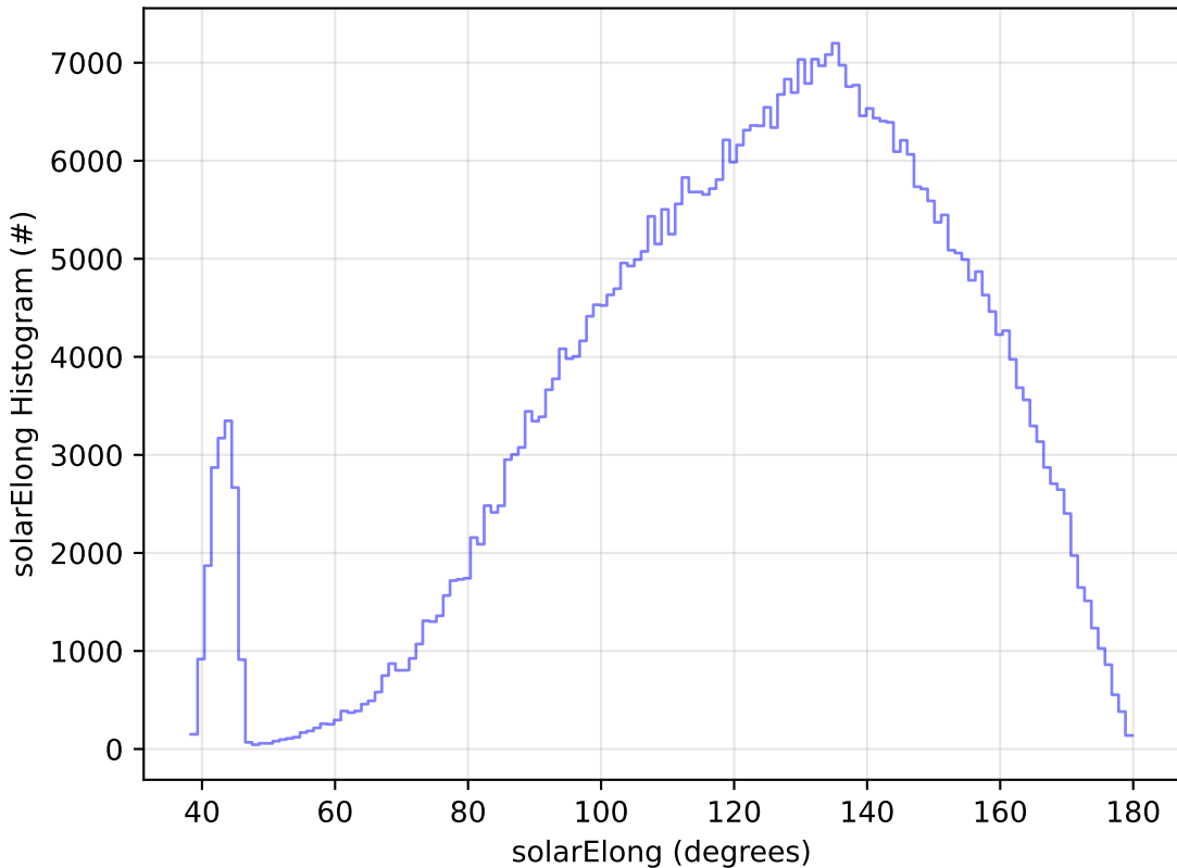
too_elab_r128_d2_griz_v3.4_10yrs All sky r band: solarElong Histogram
