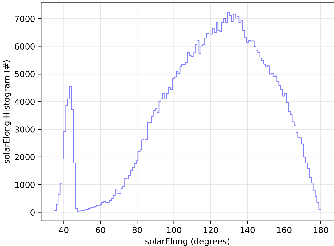
too_elab_r128_d2_griz_v3.4_10yrs All sky i band: solarElong Histogram
