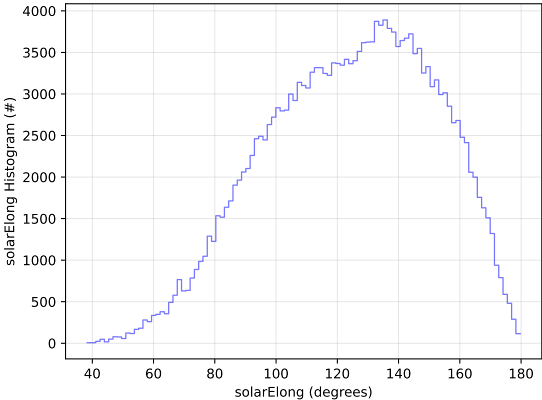
too_elab_r128_d2_griz_v3.4_10yrs All sky g band: solarElong Histogram
