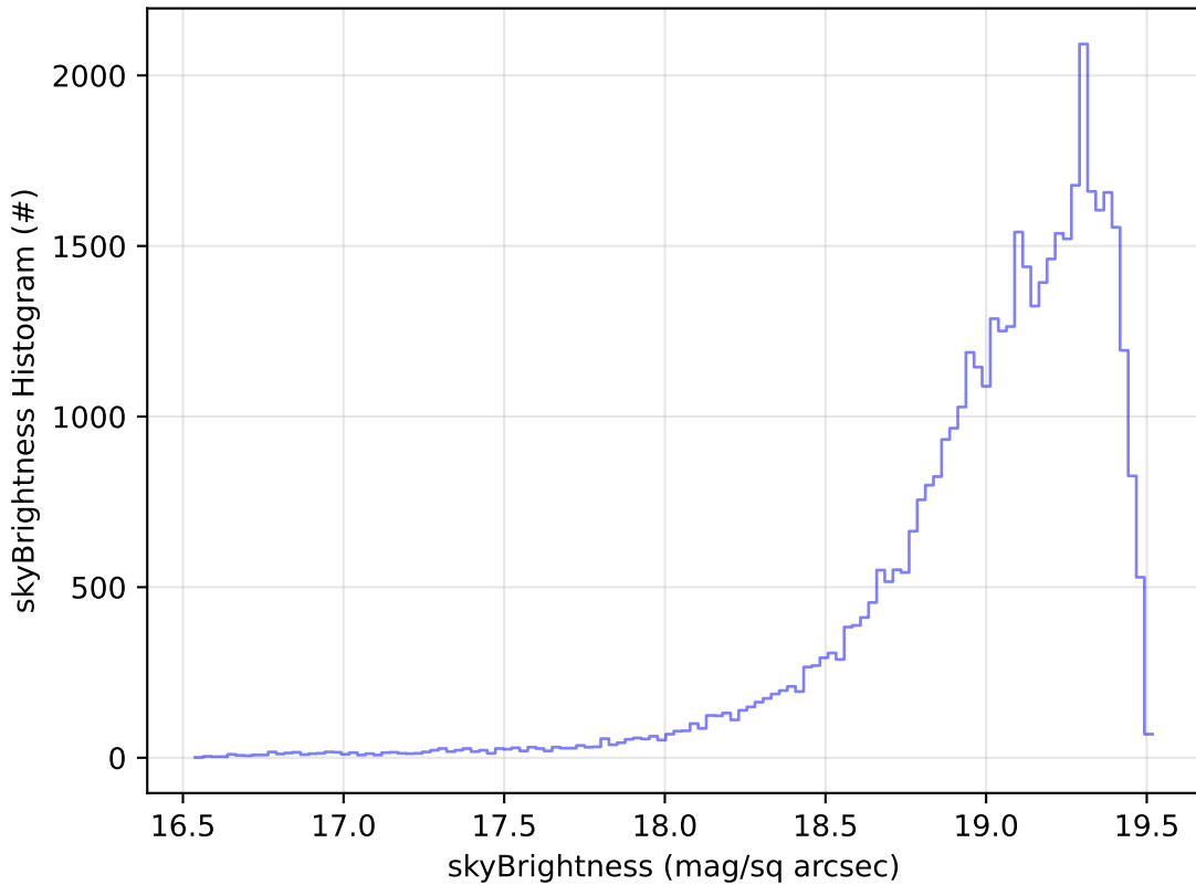
too_elab_r128_d2_griz_v3.4_10yrs Yr 1 z band: skyBrightness Histogram
