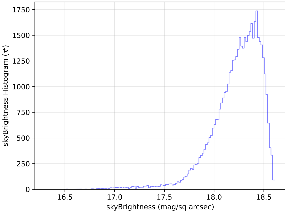
too_elab_r128_d2_griz_v3.4_10yrs Yr 1 y band: skyBrightness Histogram
