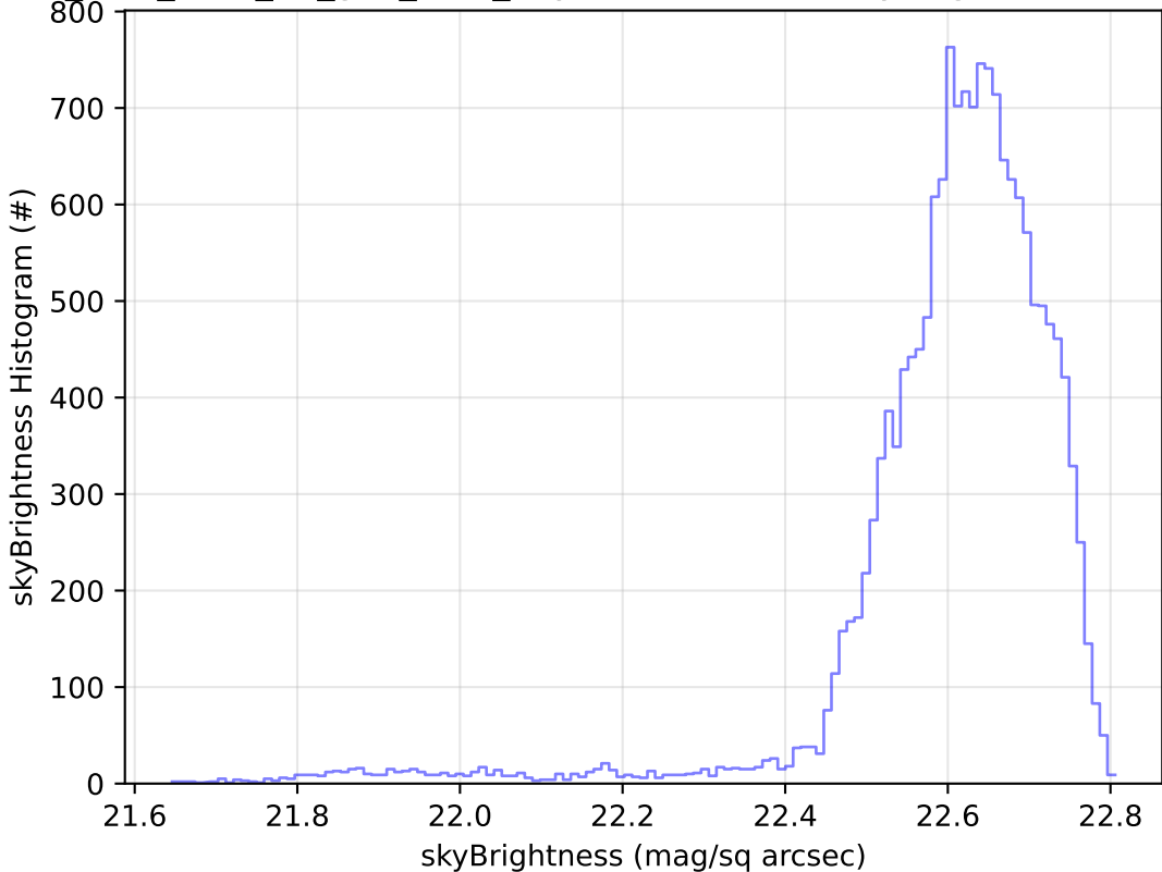
too_elab_r128_d2_griz_v3.4_10yrs Yr 1 u band: skyBrightness Histogram
