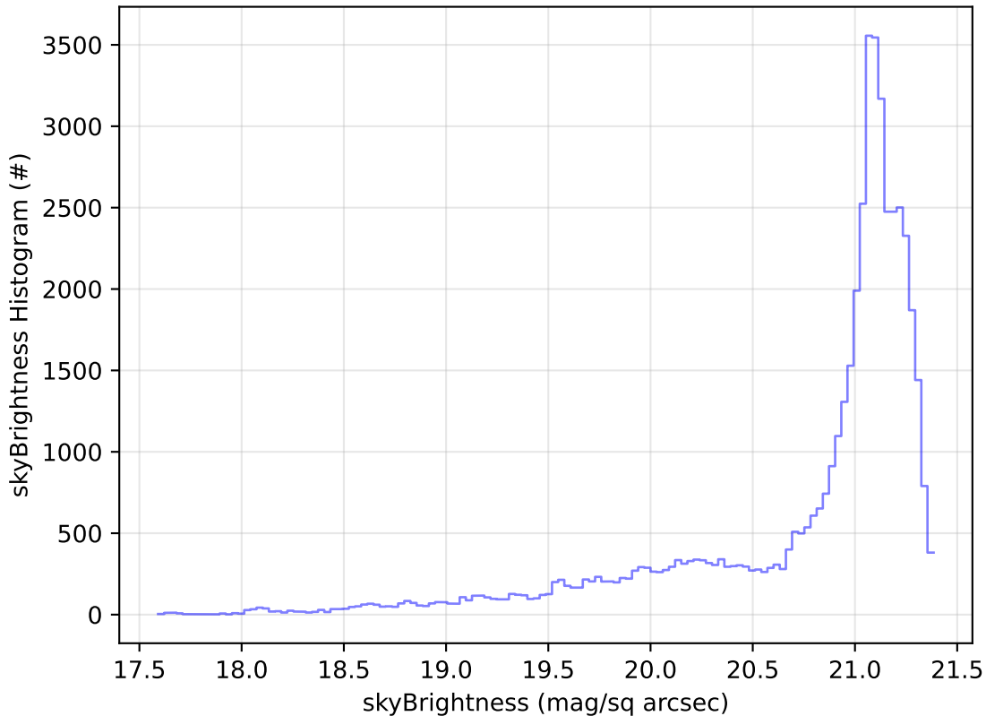
too_elab_r128_d2_griz_v3.4_10yrs Yr 1 r band: skyBrightness Histogram
