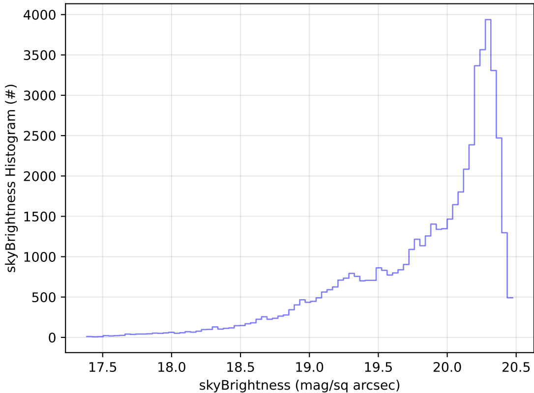
too_elab_r128_d2_griz_v3.4_10yrs Yr 1 i band: skyBrightness Histogram
