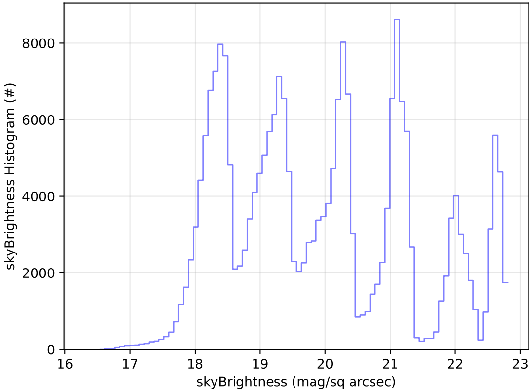
too_elab_r128_d2_griz_v3.4_10yrs Yr 1 all bands: skyBrightness Histogram
