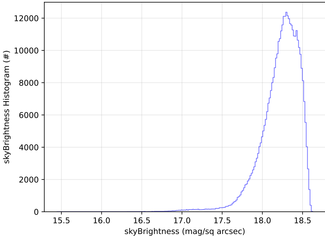
too_elab_r128_d2_griz_v3.4_10yrs WFD y band: skyBrightness Histogram
