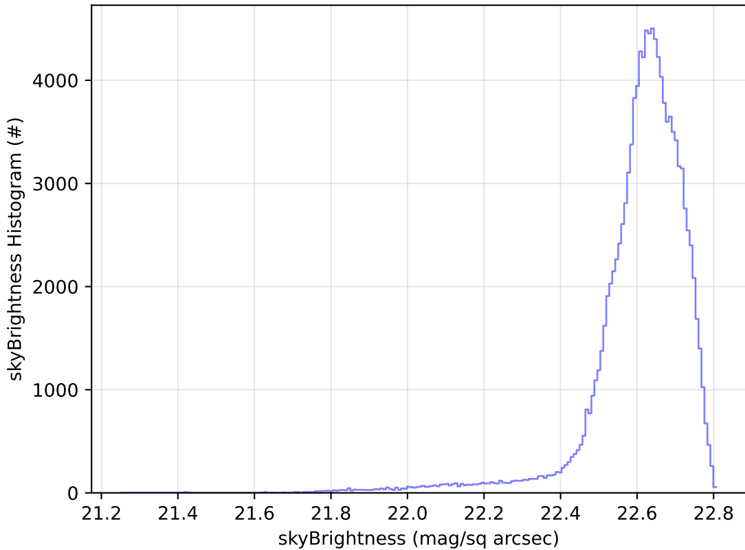
too_elab_r128_d2_griz_v3.4_10yrs WFD u band: skyBrightness Histogram
