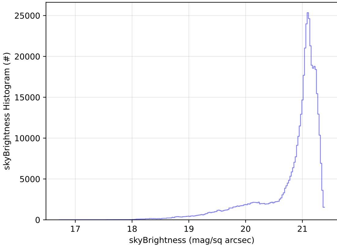
too_elab_r128_d2_griz_v3.4_10yrs WFD r band: skyBrightness Histogram
