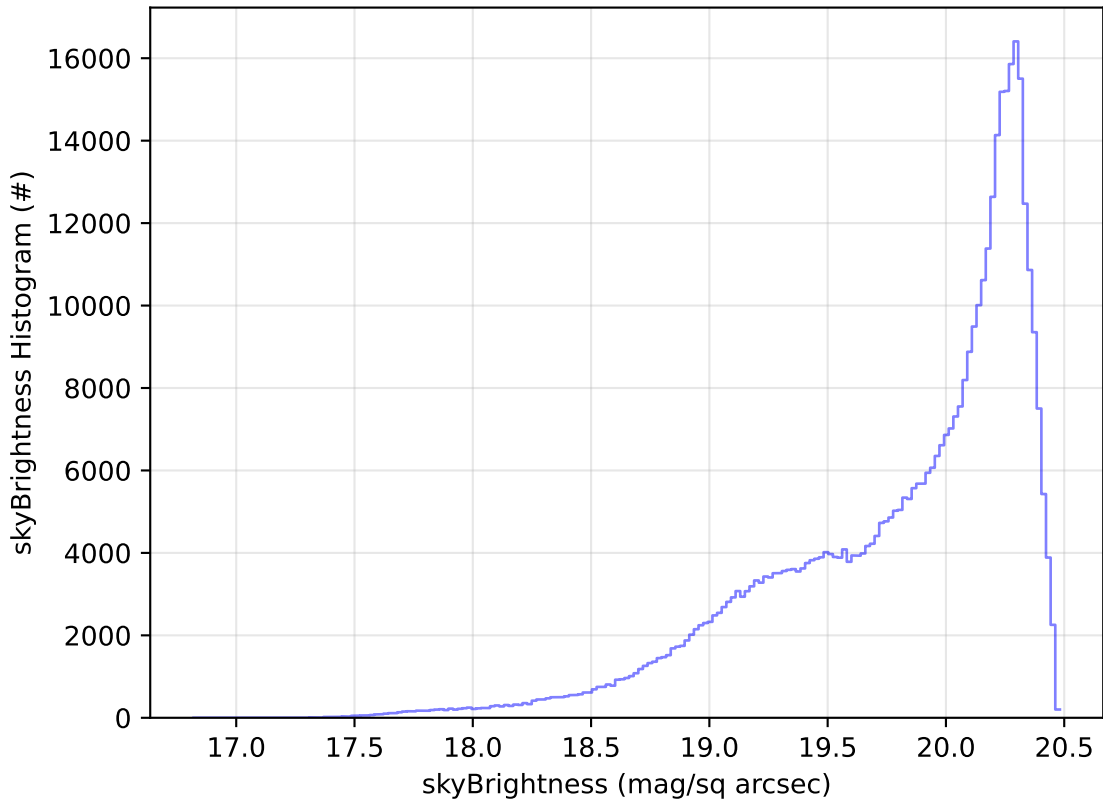
too_elab_r128_d2_griz_v3.4_10yrs WFD i band: skyBrightness Histogram
