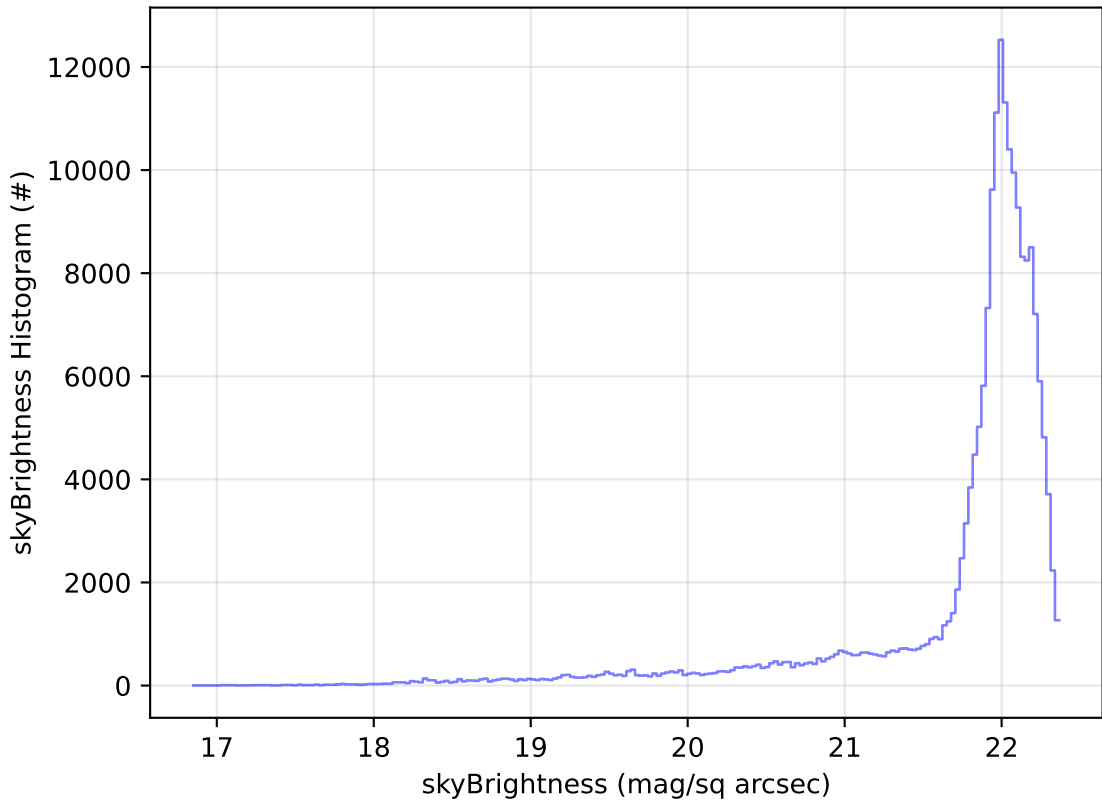
too_elab_r128_d2_griz_v3.4_10yrs WFD g band: skyBrightness Histogram
