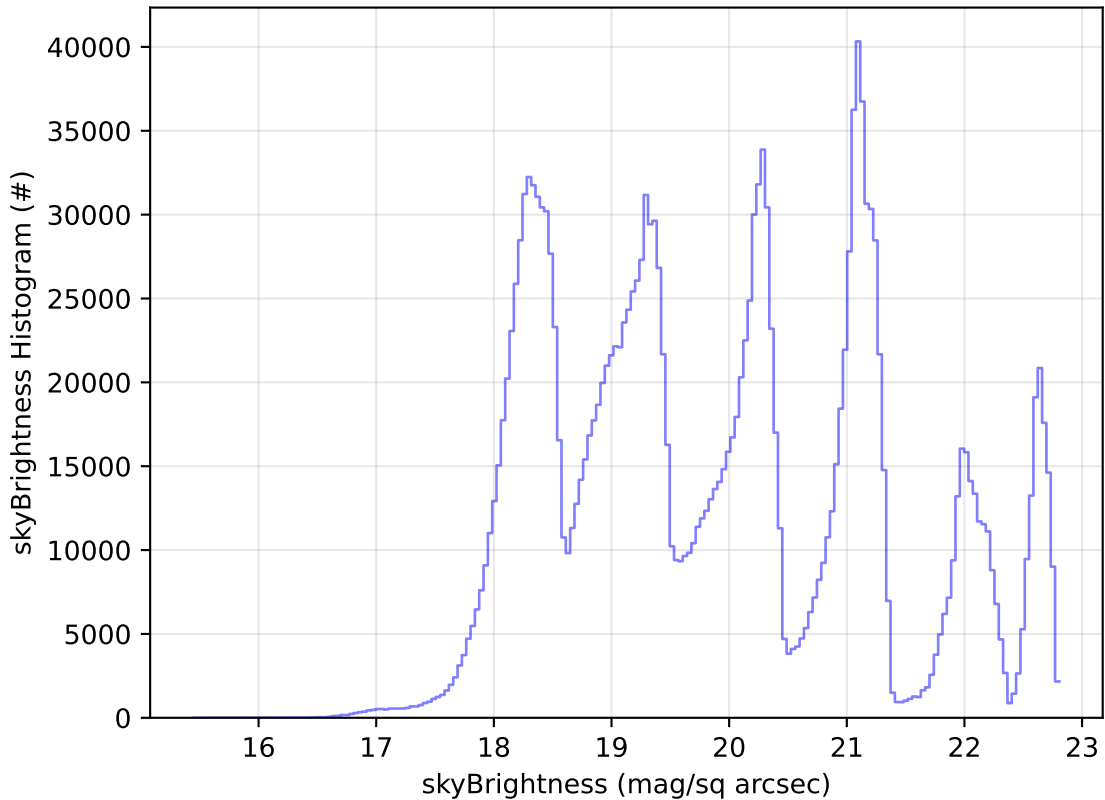
too_elab_r128_d2_griz_v3.4_10yrs WFD all bands: skyBrightness Histogram
