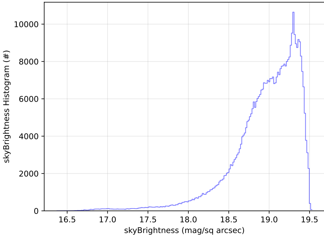
too_elab_r128_d2_griz_v3.4_10yrs All sky z band: skyBrightness Histogram
