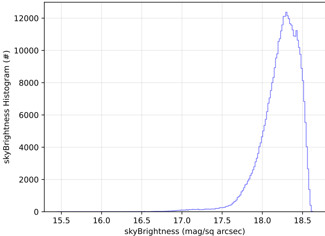
too_elab_r128_d2_griz_v3.4_10yrs All sky y band: skyBrightness Histogram
