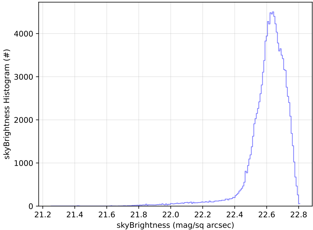
too_elab_r128_d2_griz_v3.4_10yrs All sky u band: skyBrightness Histogram
