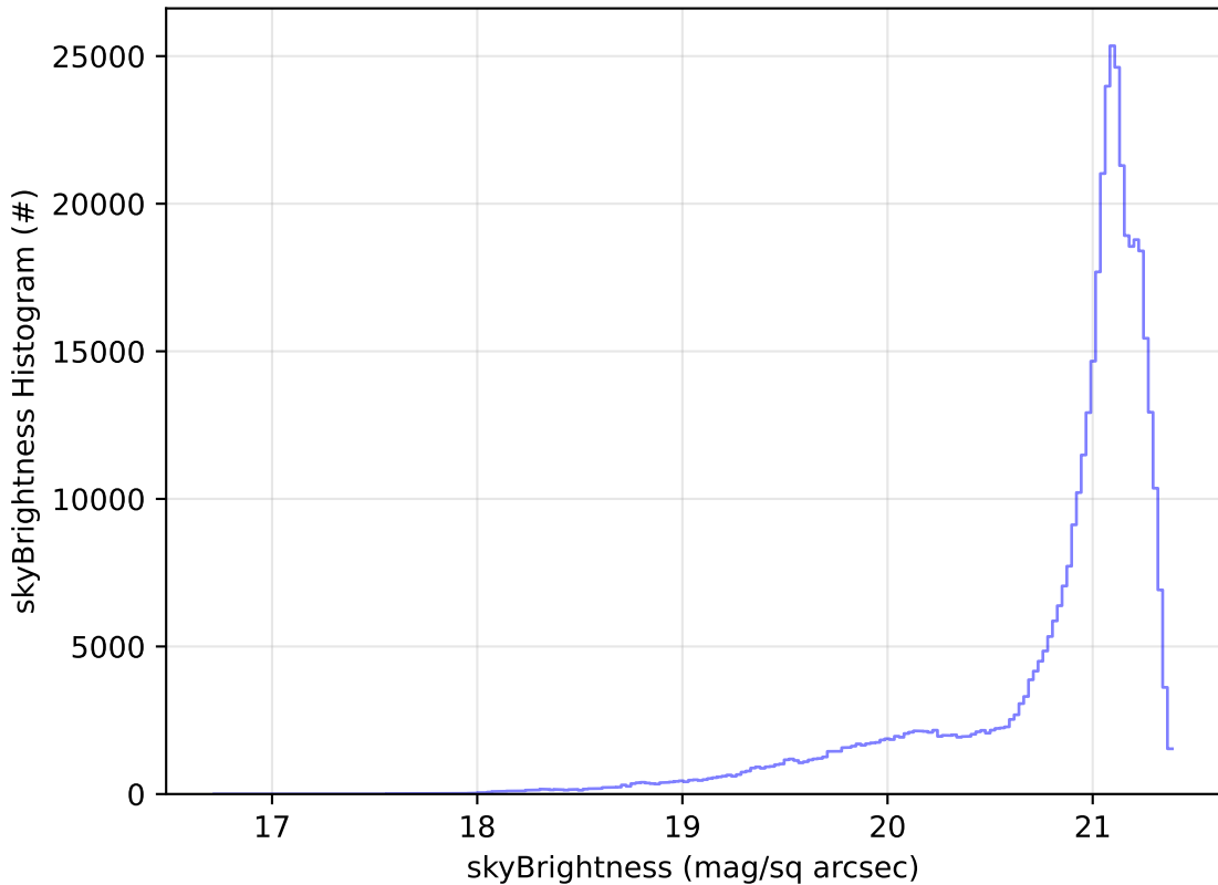
too_elab_r128_d2_griz_v3.4_10yrs All sky r band: skyBrightness Histogram
