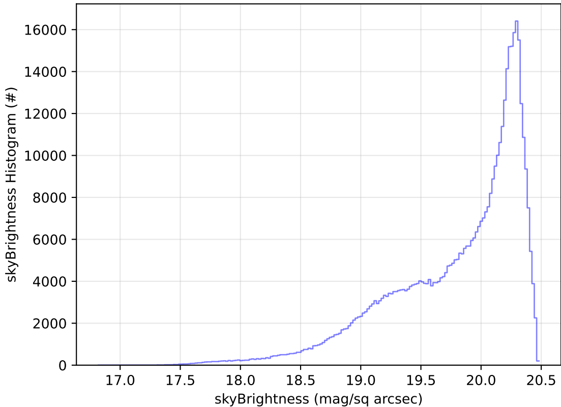
too_elab_r128_d2_griz_v3.4_10yrs All sky i band: skyBrightness Histogram
