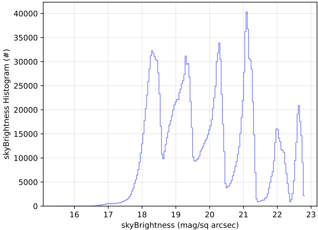
too_elab_r128_d2_griz_v3.4_10yrs All sky all bands: skyBrightness Histogram
