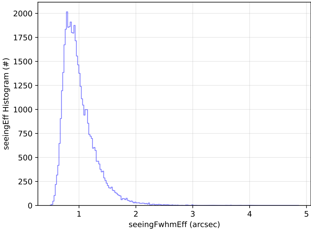
too_elab_r128_d2_griz_v3.4_10yrs Yr 1 z band: seeingEff Histogram
