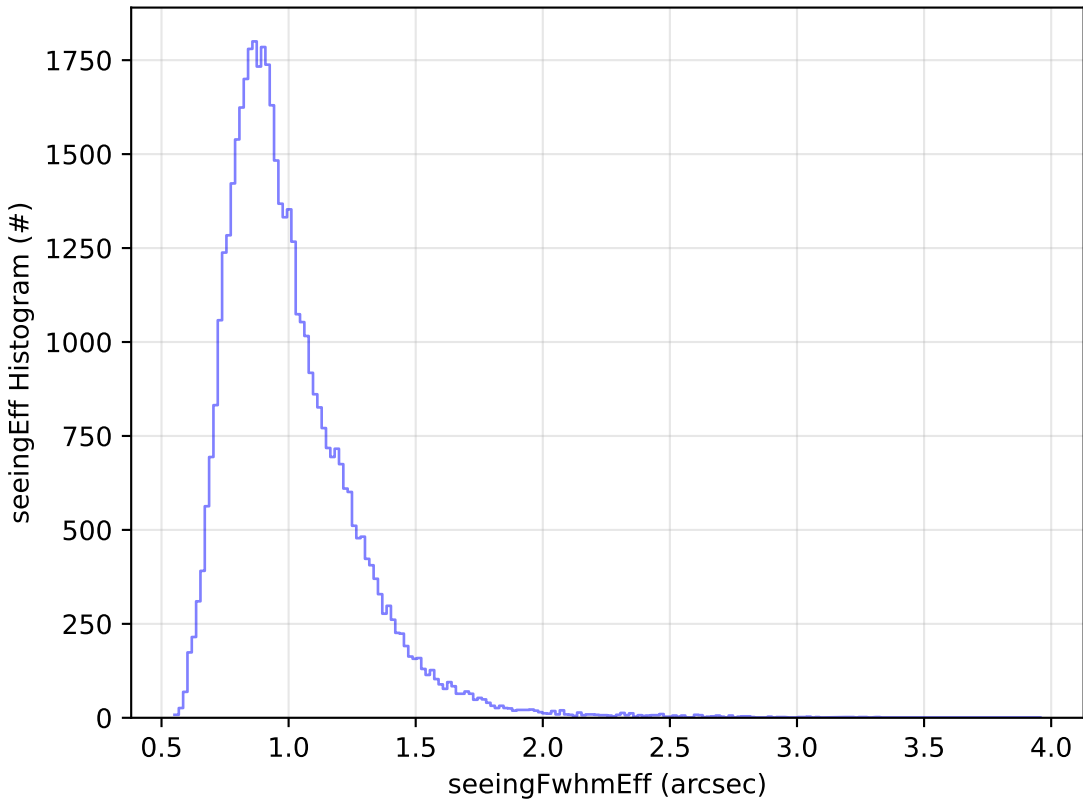
too_elab_r128_d2_griz_v3.4_10yrs Yr 1 y band: seeingEff Histogram
