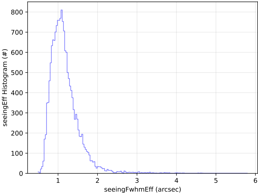
too_elab_r128_d2_griz_v3.4_10yrs Yr 1 u band: seeingEff Histogram
