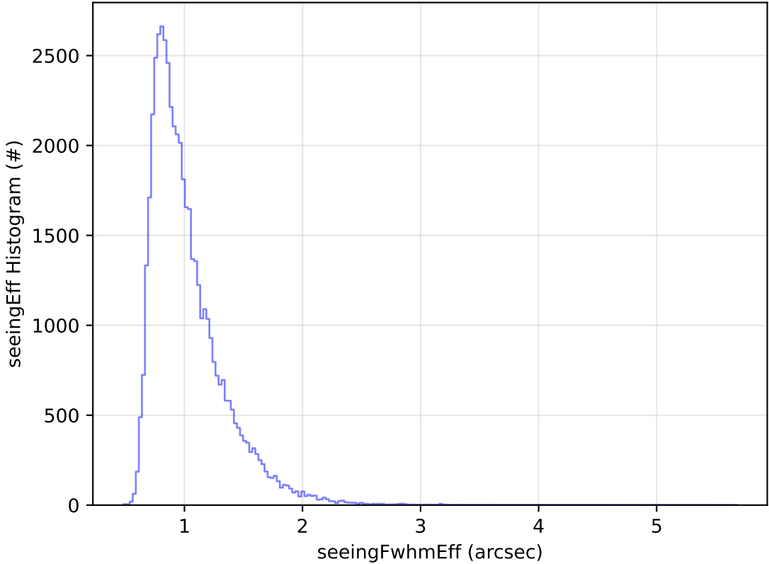
too_elab_r128_d2_griz_v3.4_10yrs Yr 1 r band: seeingEff Histogram
