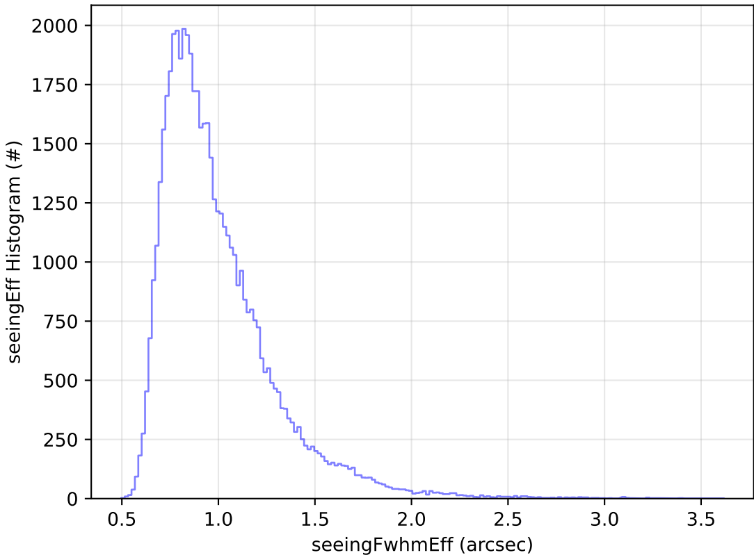
too_elab_r128_d2_griz_v3.4_10yrs Yr 1 i band: seeingEff Histogram
