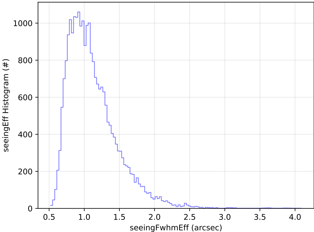
too_elab_r128_d2_griz_v3.4_10yrs Yr 1 g band: seeingEff Histogram
