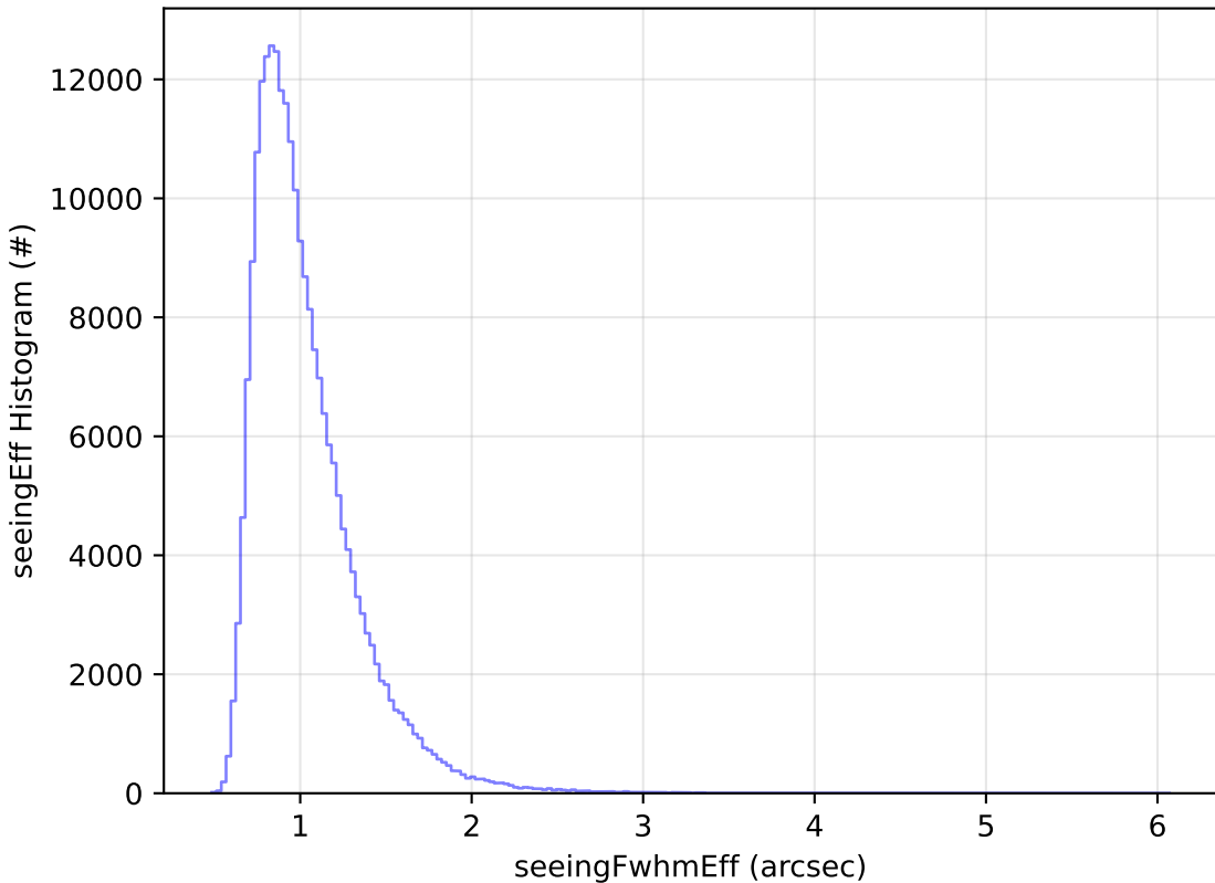
too_elab_r128_d2_griz_v3.4_10yrs Yr 1 all bands: seeingEff Histogram
