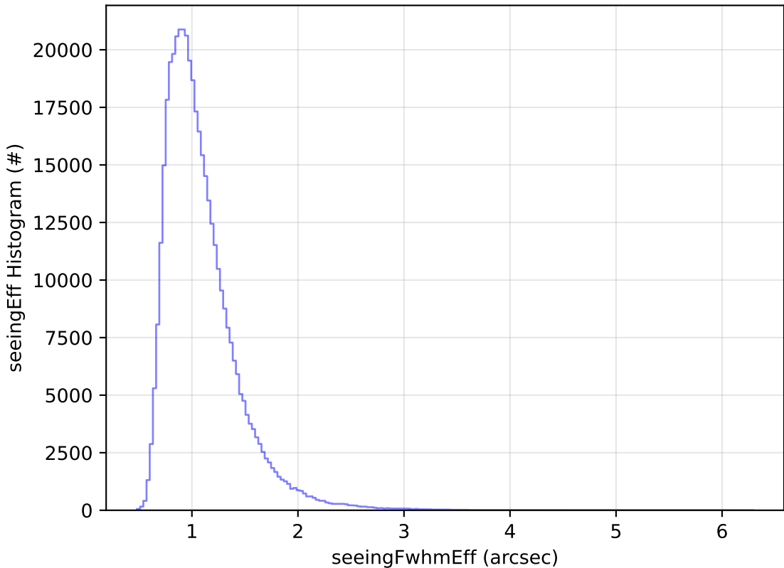
too_elab_r128_d2_griz_v3.4_10yrs WFD z band: seeingEff Histogram
