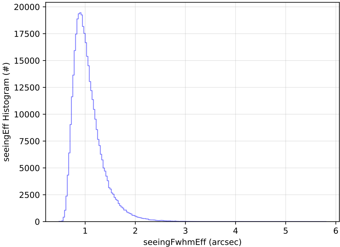
too_elab_r128_d2_griz_v3.4_10yrs WFD y band: seeingEff Histogram
