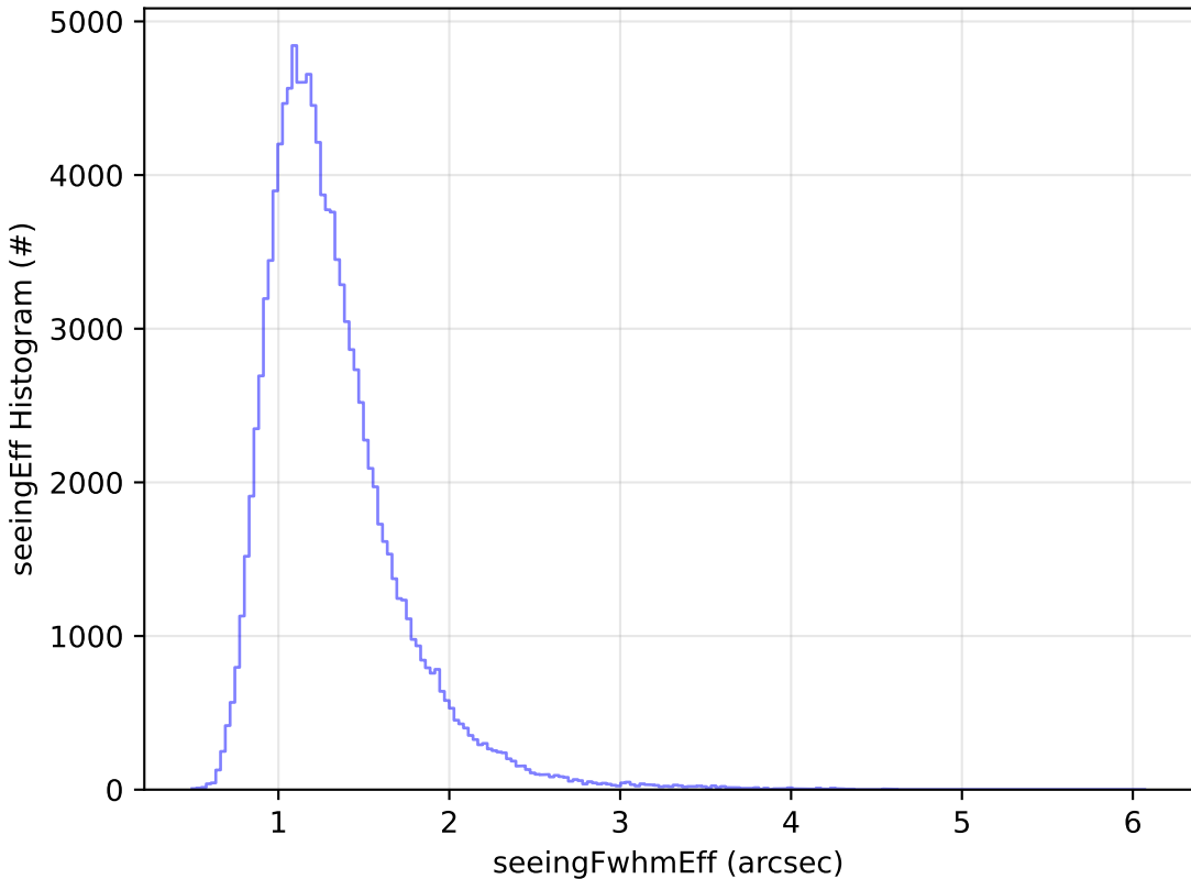
too_elab_r128_d2_griz_v3.4_10yrs WFD u band: seeingEff Histogram
