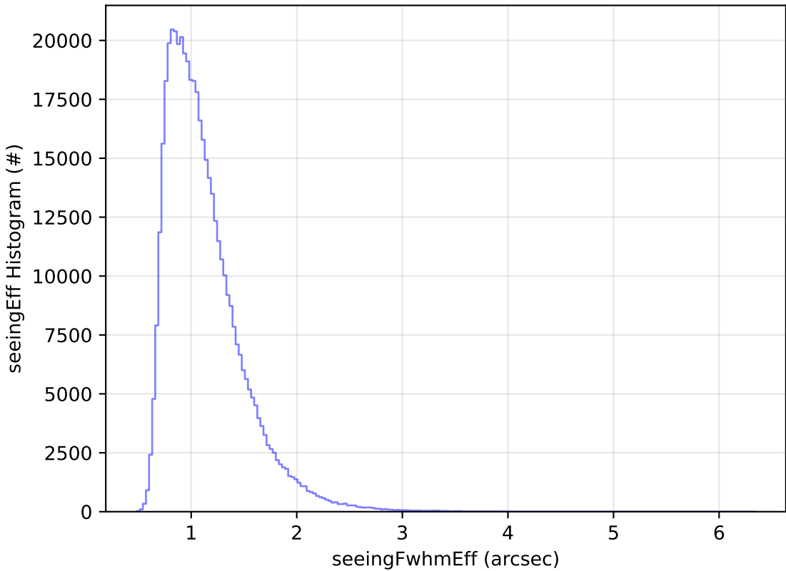
too_elab_r128_d2_griz_v3.4_10yrs WFD r band: seeingEff Histogram
