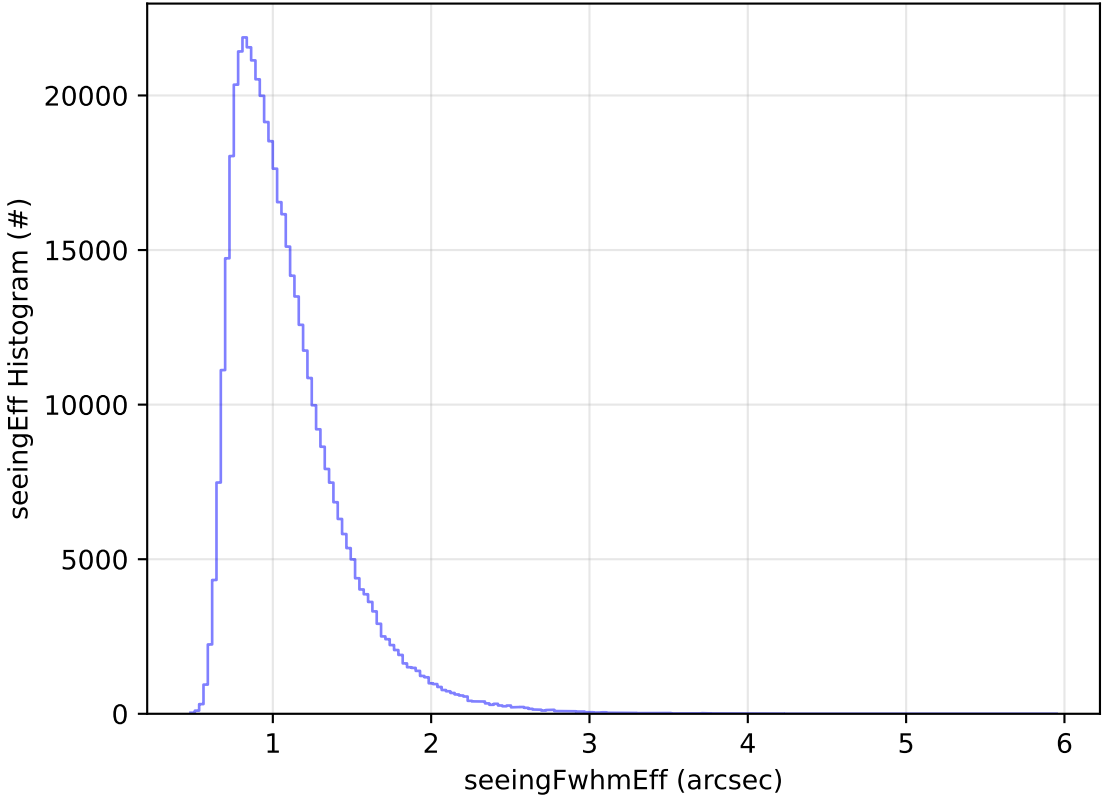
too_elab_r128_d2_griz_v3.4_10yrs WFD i band: seeingEff Histogram
