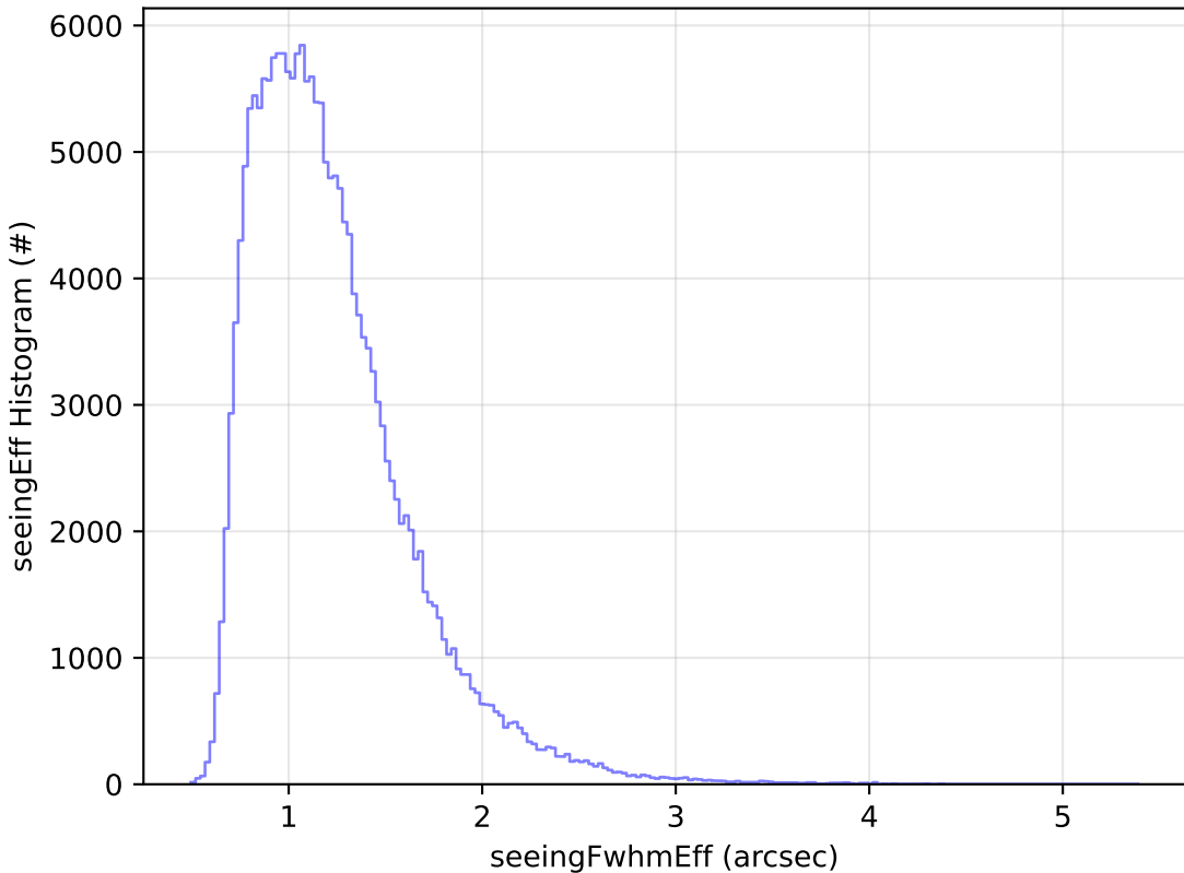
too_elab_r128_d2_griz_v3.4_10yrs WFD g band: seeingEff Histogram
