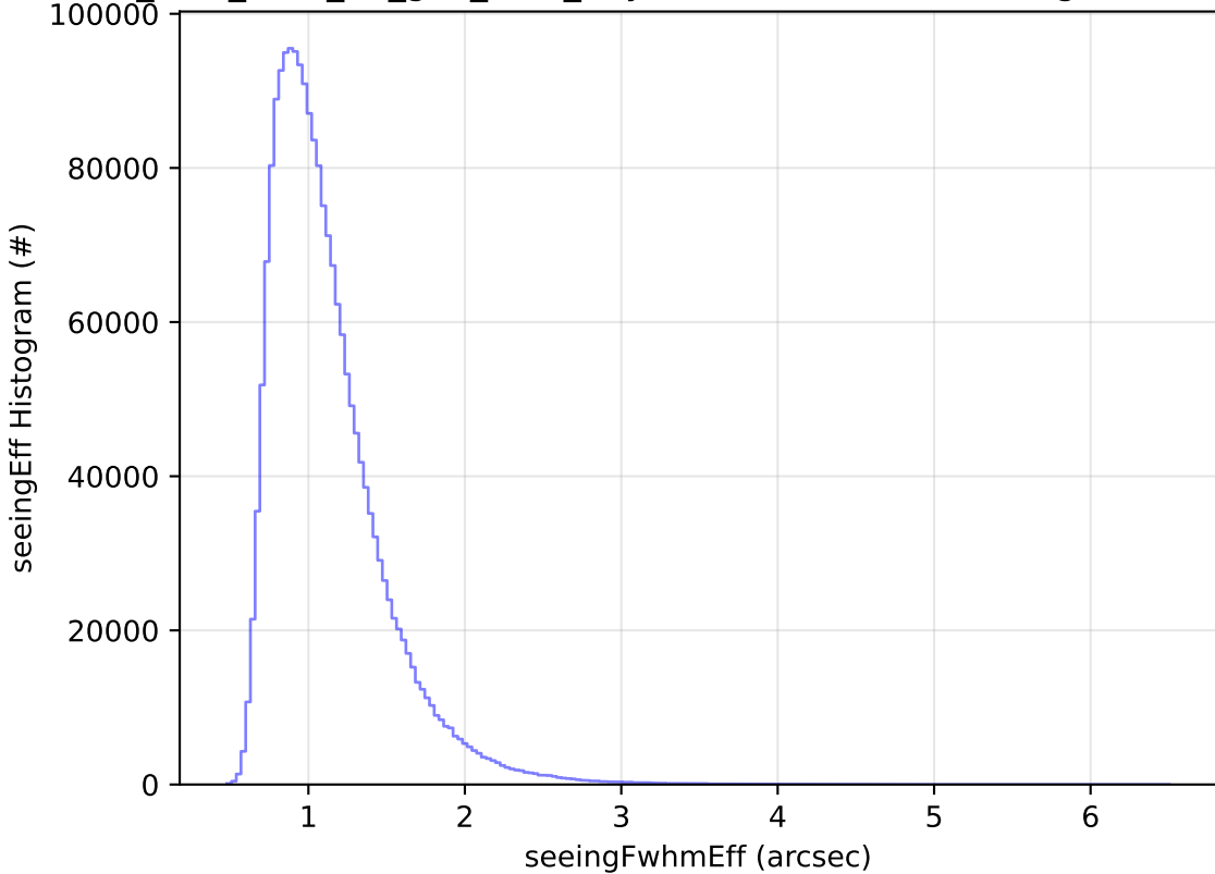
too_elab_r128_d2_griz_v3.4_10yrs WFD all bands: seeingEff Histogram
