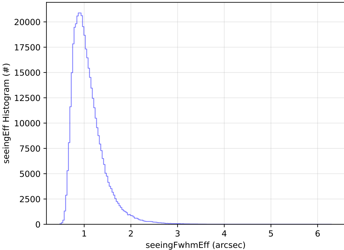
too_elab_r128_d2_griz_v3.4_10yrs All sky z band: seeingEff Histogram
