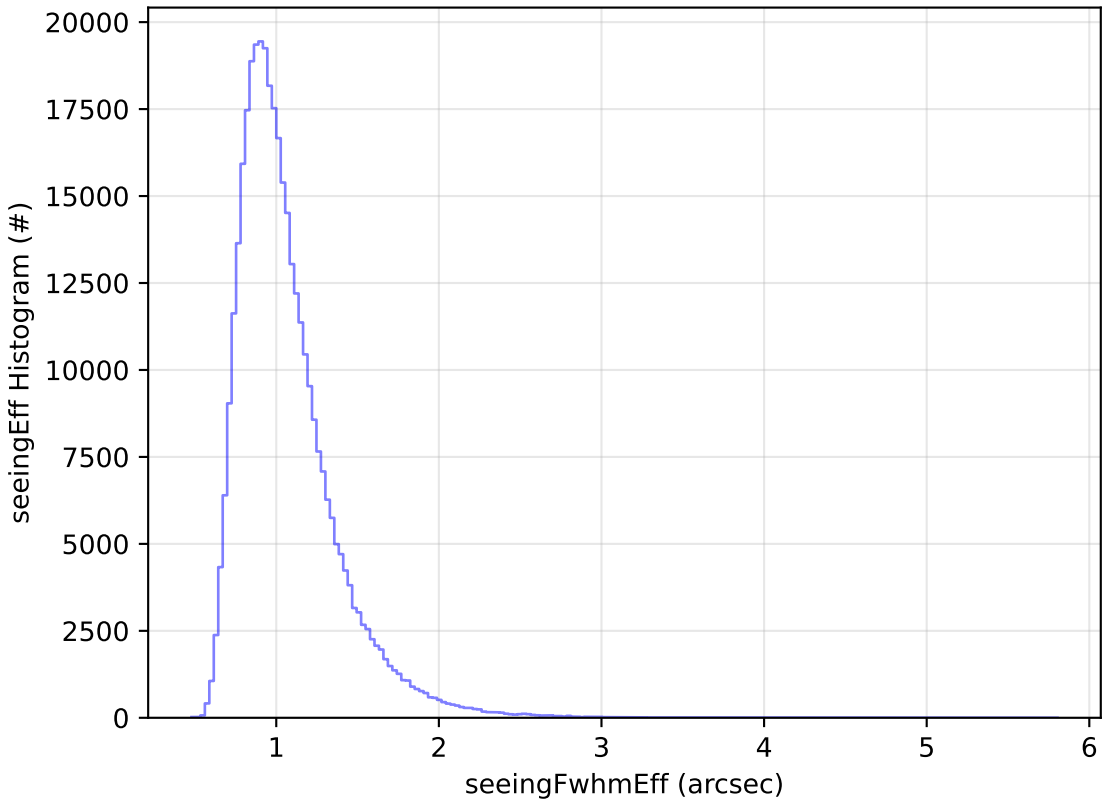
too_elab_r128_d2_griz_v3.4_10yrs All sky y band: seeingEff Histogram
