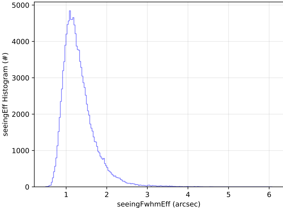
too_elab_r128_d2_griz_v3.4_10yrs All sky u band: seeingEff Histogram
