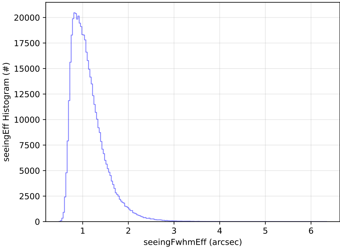
too_elab_r128_d2_griz_v3.4_10yrs All sky r band: seeingEff Histogram
