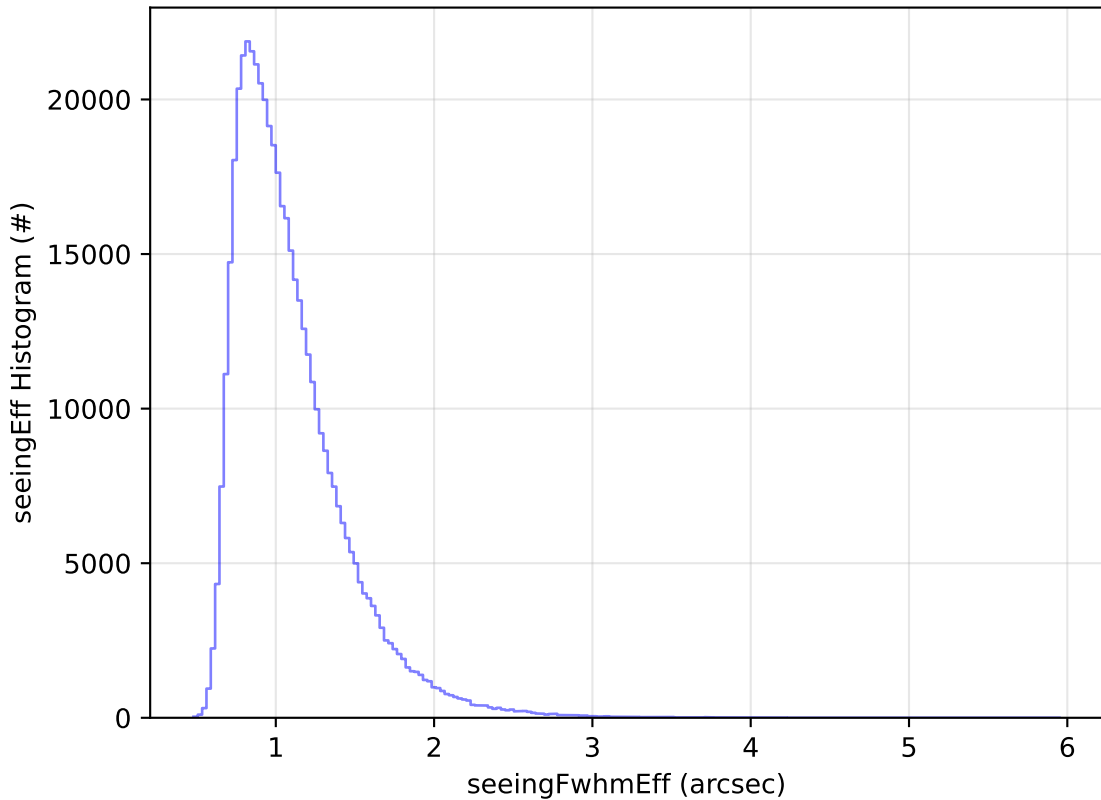
too_elab_r128_d2_griz_v3.4_10yrs All sky i band: seeingEff Histogram
